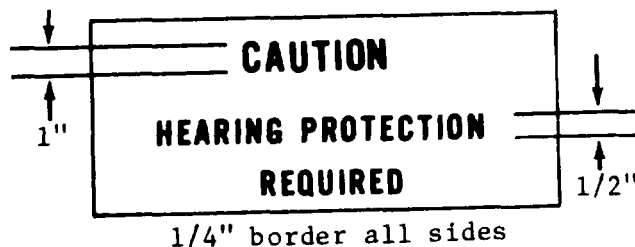
Figure 7-2. Size and Wording of Stencil
