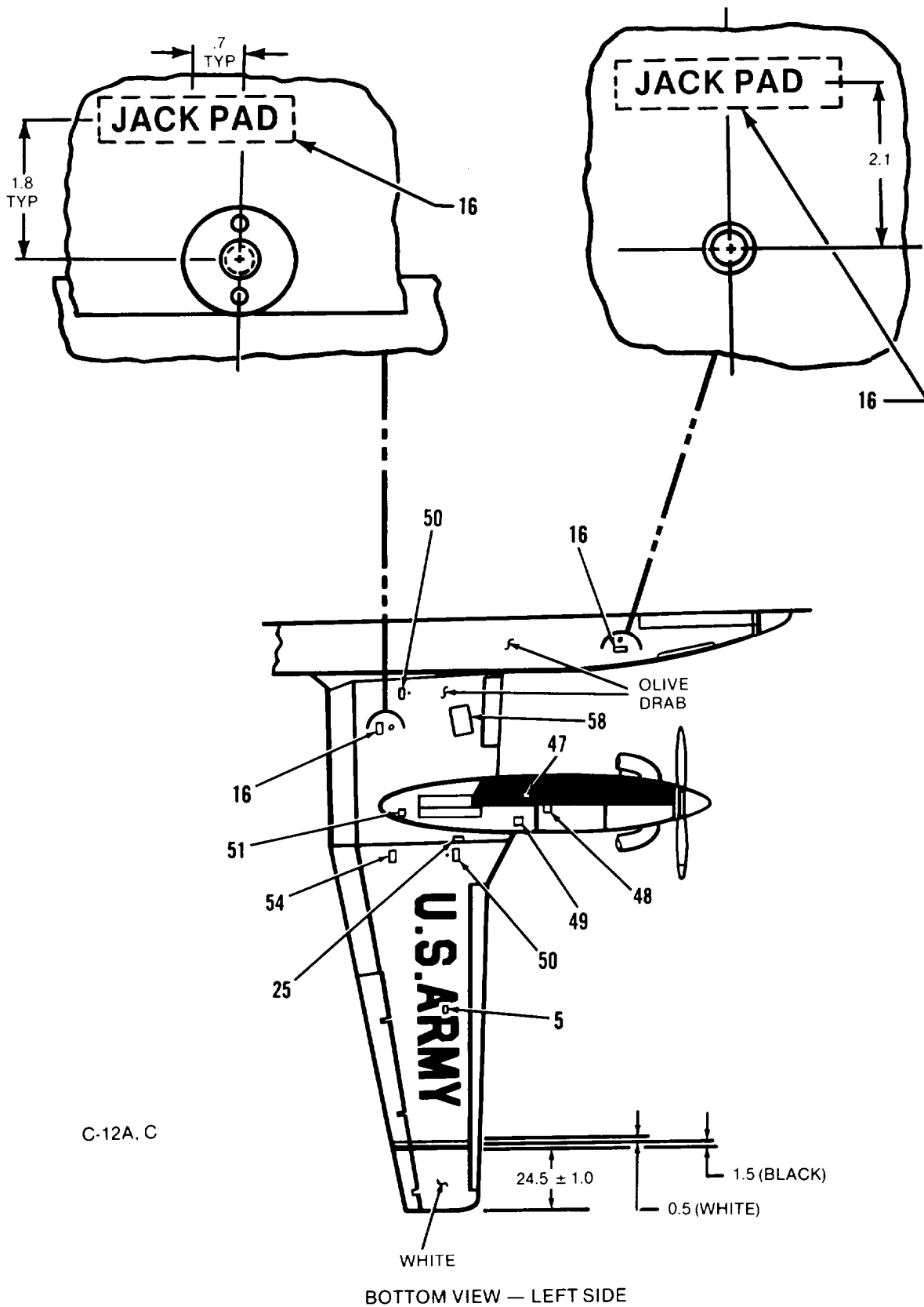
Figure 10-1. Exterior Markings, C-12 (Sheet 4 of 27)
