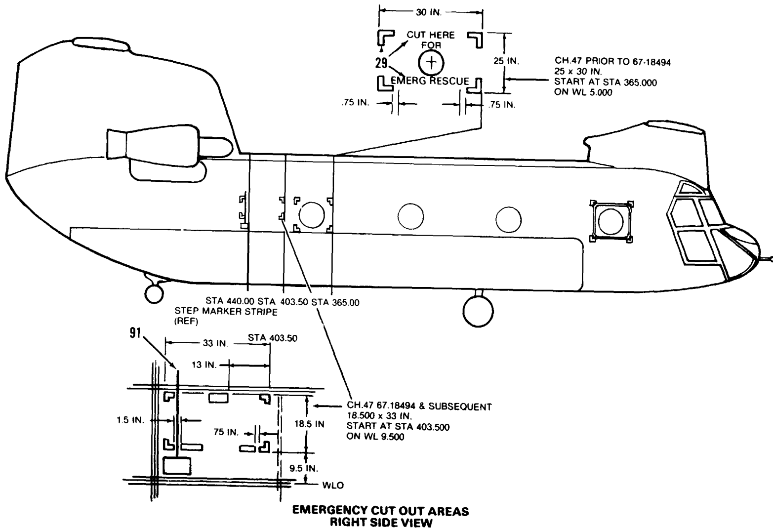
Figure 9-10. Exterior Markings, CH- 47 (Sheet 11 of 29)
