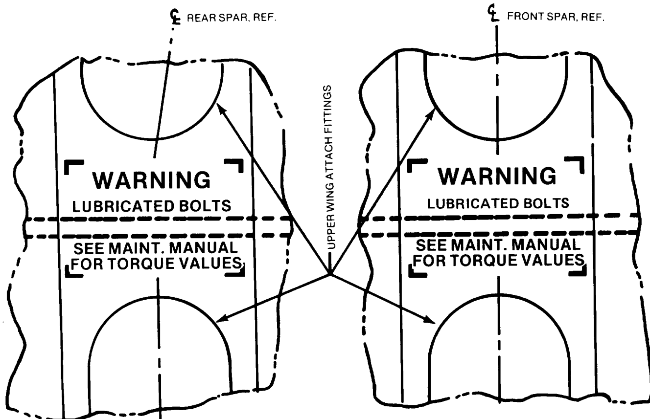
DETAIL A: WING ATTACH FITTINGS, LEFT HAND SHOWN, RIGHT HAND OPPOSITE, FITTING COVERS OMITTED.
