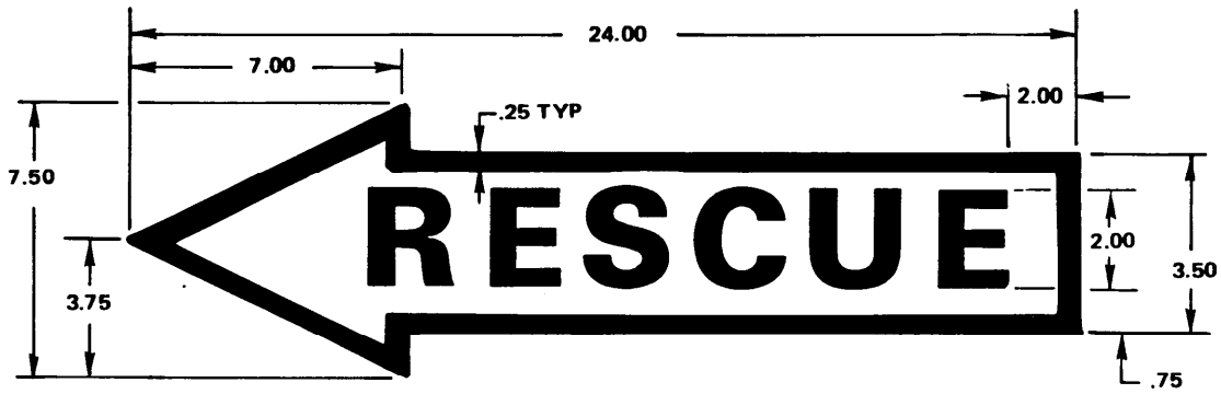
FIGURE A-12. Helicopter tail boom markings.
