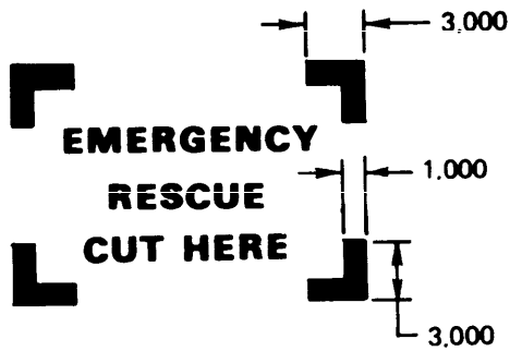
CORNER MARKING DIMENSIONS IN INCHES
