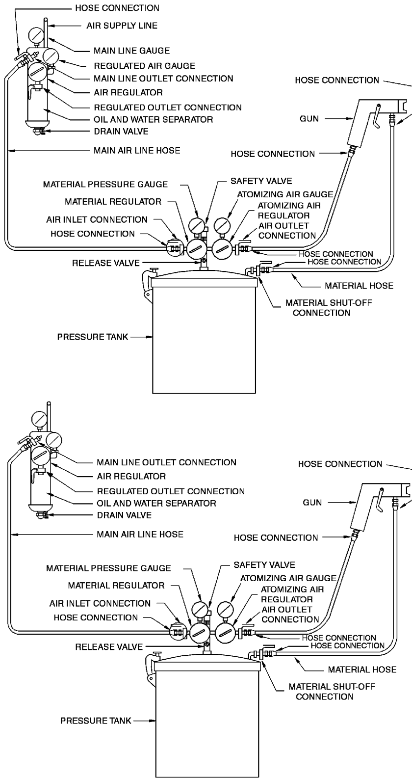
Figure 4-2. Simple Spray System Setup
