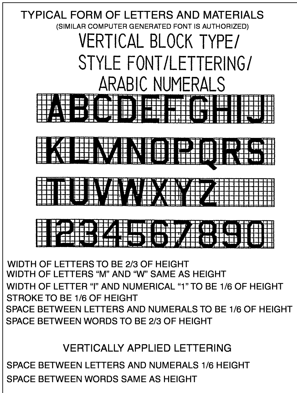
Figure B-3. Form of Letters and Numerals
